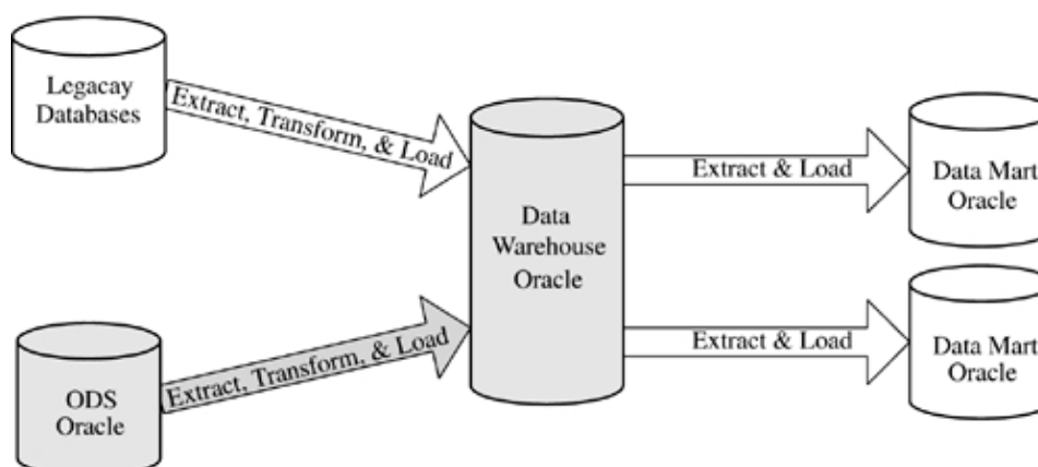
Figure 1-2. Typical Data Warehouse Data Loading Options
